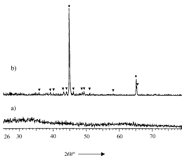
Figure 1. XRD diagrams of as-prepared (a) and annealed materials (b). ♦ bcc Fe, ▼ \text{Fe}_3\text{C} .
